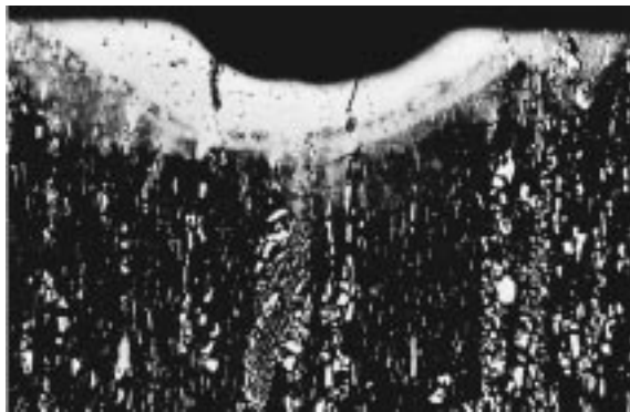
Fig 8. A section through one of the suspected "pores".
