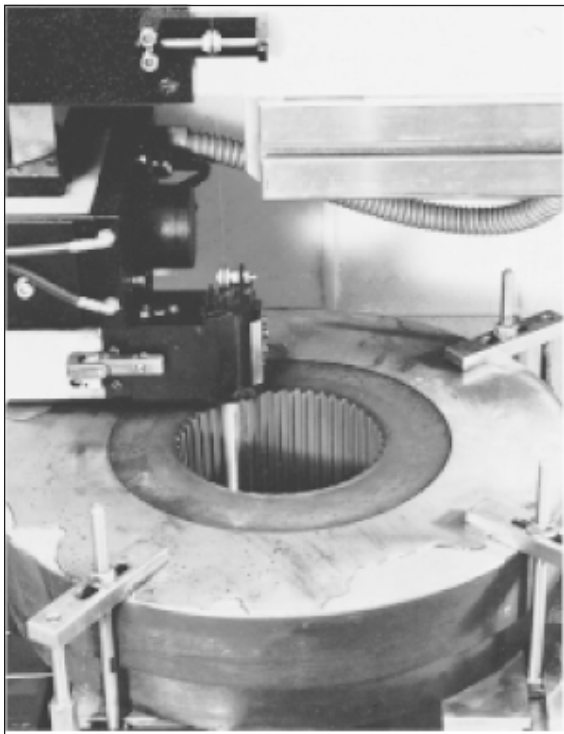
Fig. 11. Wire erosion of a hardened and tempered tool steel blanking die.
