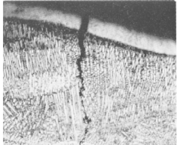
Fig. 3. Pillar crystals formed during solidification.
