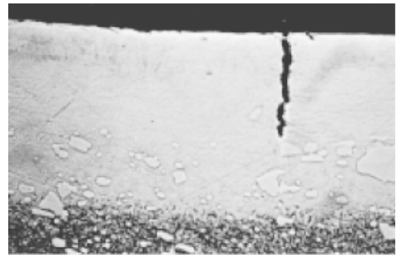
Fig. 6e. Graphite electrode. t_1 = 500 \mu\text{s} . Magnification 500 X
