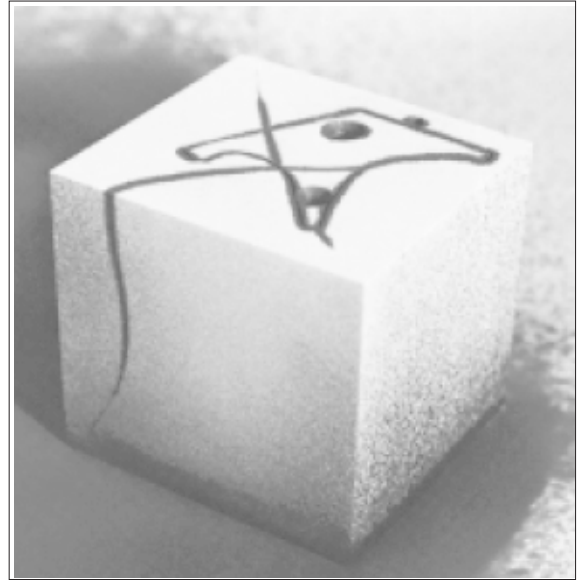
Fig. 12. This block of D2 steel, approx. 50 x 50 x 50 mm (2" x 2" x 2"), cracked during the wire EDM operation.
