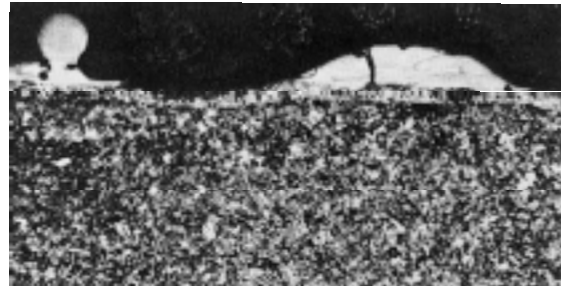
Fig. 1. A “rough-machined” EDM surface with a cross section through chips and craters. Material: ORVAR 2 Microdized.
